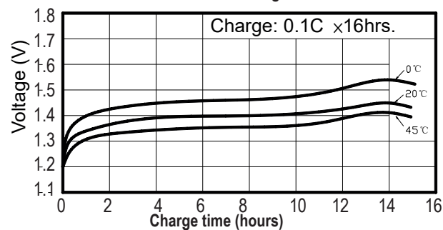
Typical characteristics Standard Charge
