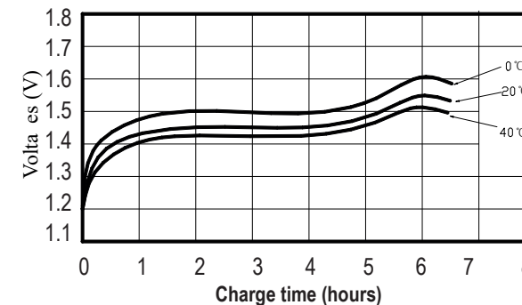
Rapid charge Charge: 0.2Cx6hrs
