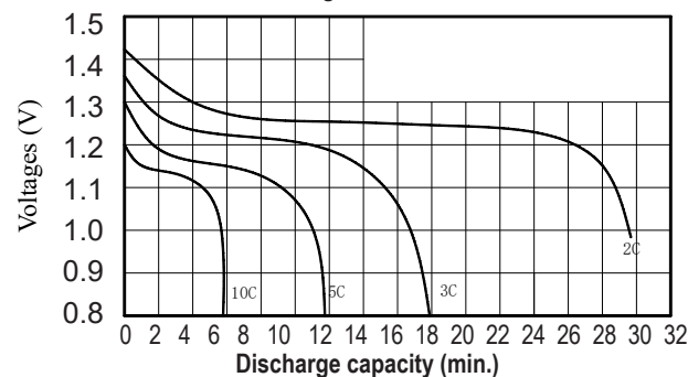
Discharge characteristics
